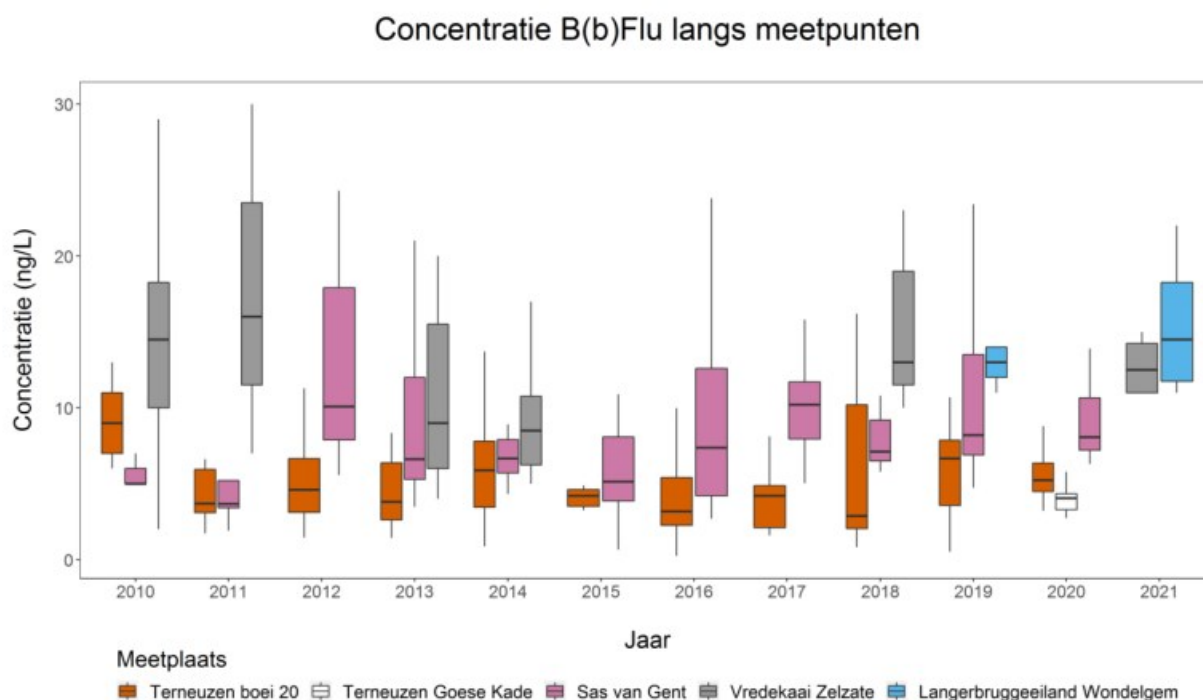
Figuur 51: B(b)F – Verloop gemeten concentratie doorheen studiegebied.
