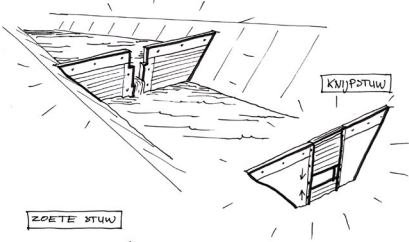
STUW
