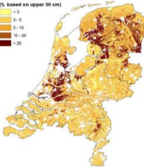
Soil organic matter content (% based on upper 30 cm)
