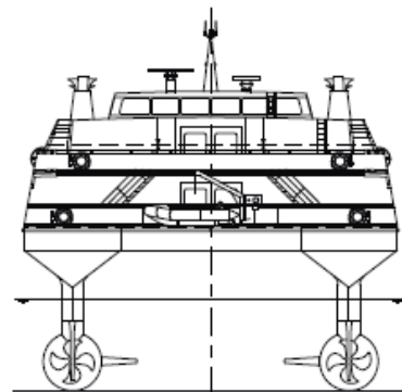
Stern View
