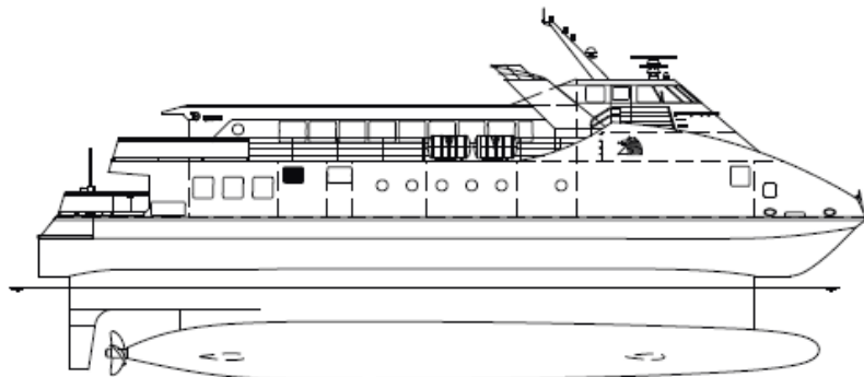
Outboard Profile
